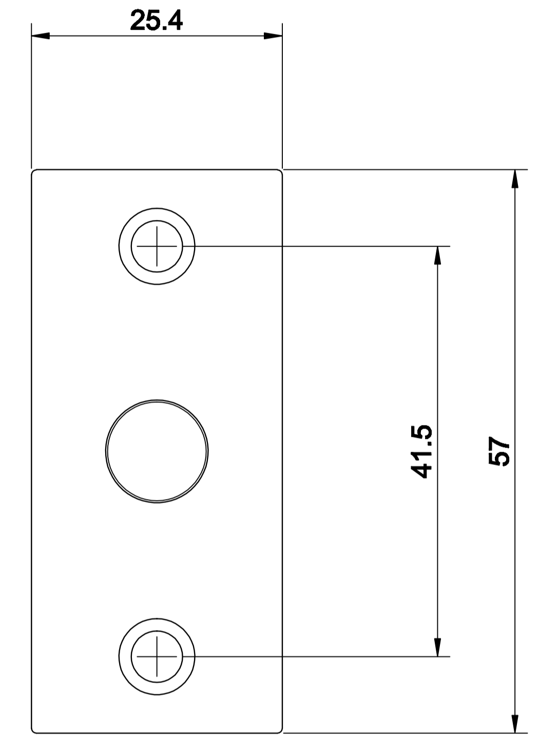
1.2mm Brass Face Plate
